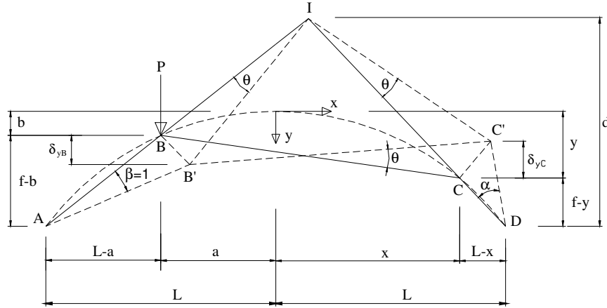
Figure 2: Collapse mechanism for the arch carrying a point load P
