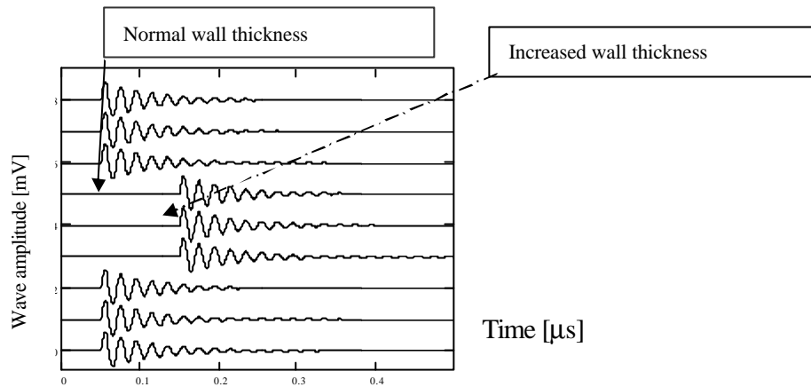
Figure 5: Example of change in travel time because of changes in wall thickness
