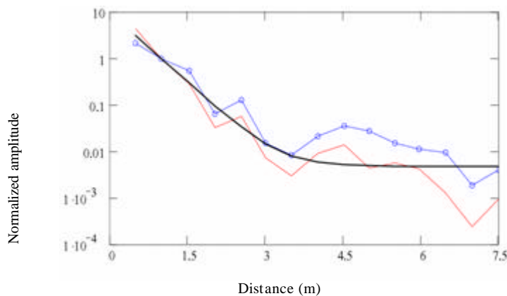
Figure 7: Normalized attenuation of maximum response in time and frequency
