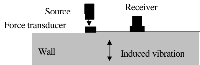
Figure 2: Impulse-response test method
