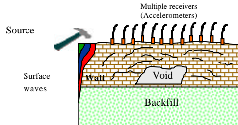
Figure 6: Example of multi-channel array of transducers
