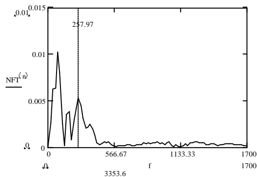
Figure 8. Fourier spectra for the signal of receiver 1
