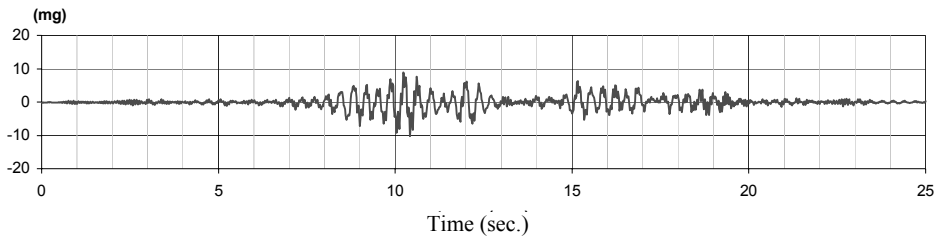
Figure 10 : Longitudinal acceleration in the reference point 24
