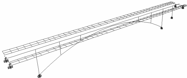
Figure 4 : The numeric model
