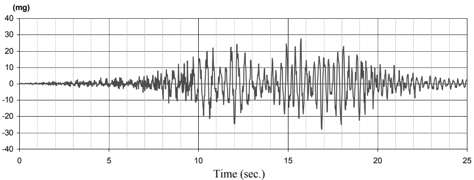
Figure 9 : Vertical acceleration in the reference point 9
