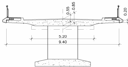
Figure 3 : The deck transverse section
