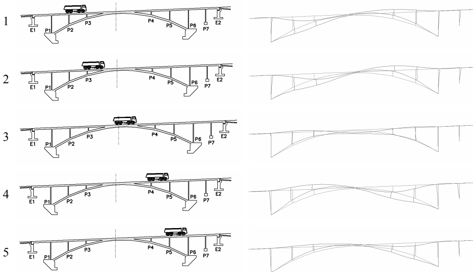
Figure 6 : Load positions and structural deformation
