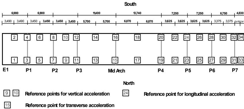
Figure 8 : Instrumented points in the dynamic tests
