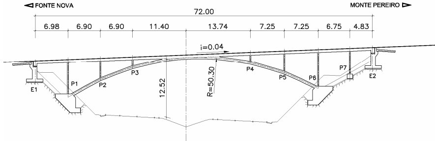
Figure 2 : Elevation view
