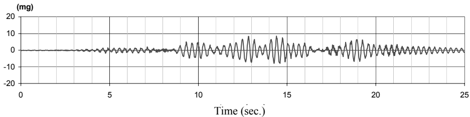
Figure 11 : Transverse acceleration in the reference point 15
