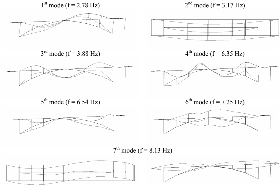
Figure 13 : Identified mode shapes
